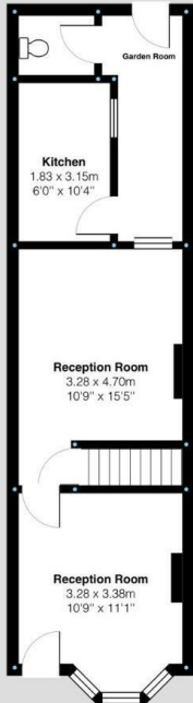
Ground Floor
